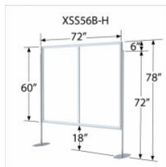
Center Spanner Support Bars are available for spans greater than 48"
