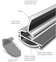
GCO GRIPGRAPHIC ANATOMY
